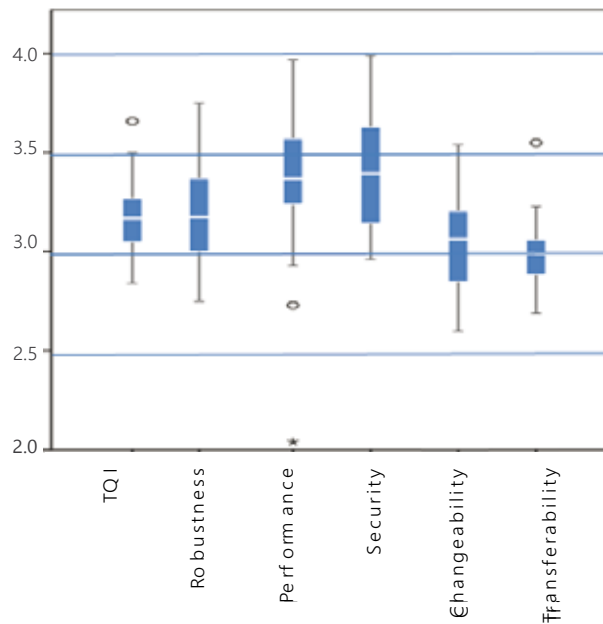
Figure 12. Box and whisker plots for TQI and health factors in C++
