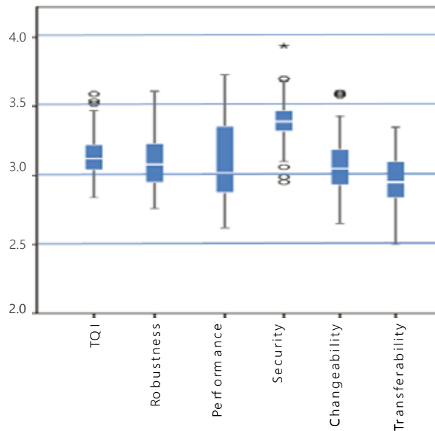
Figure 8. Box and whisker plots for TQI and health factors in ABAP
